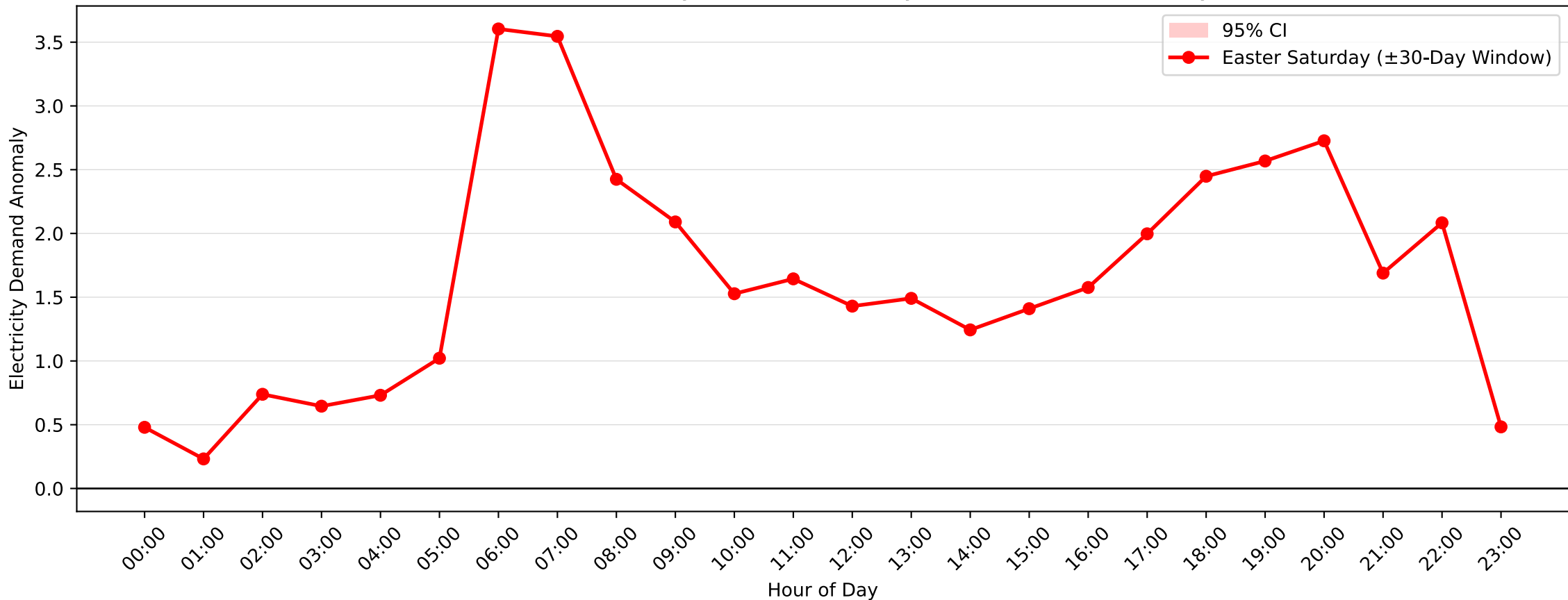
Beacon Hill Demand Anomaly: Easter Saturday (2004-2005, \pm 30 -Day Window)
