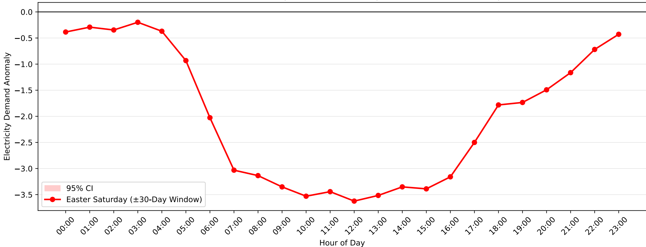
Beacon Hill Demand Anomaly: Easter Saturday (2017-2018, \pm 30 -Day Window)
